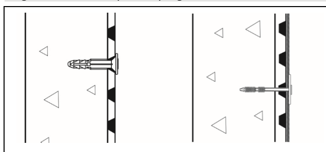
Figure 2 Brick and plaster plug
